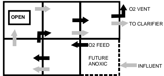
Figure 9B New Reactor No. 3, Morganton, NC
