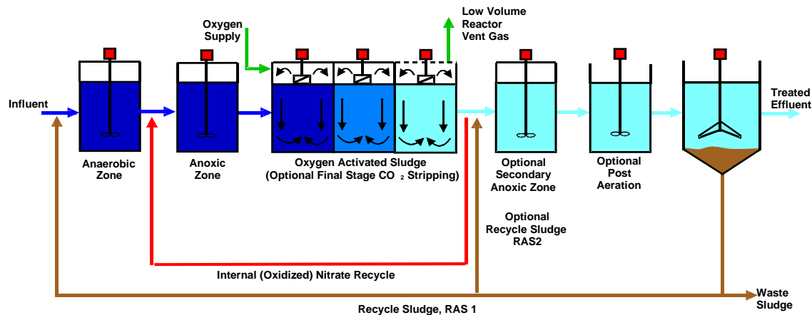
FIGURE 7 UNOX BNR Systems Process Flow Schematic
