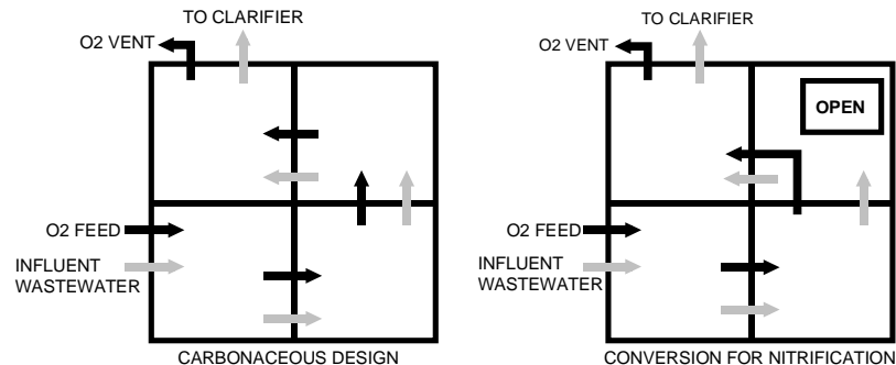
Figure 9A Reactor Modifications, Morganton, NC
