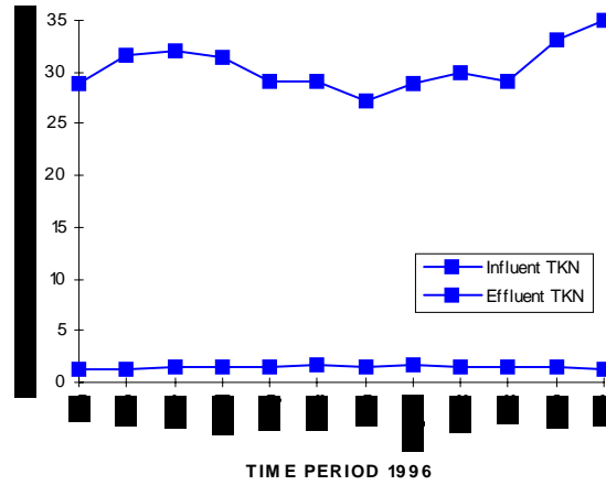
•FIGURE 5B •Tampa, FL 2 Step Nitrification •1996 Monthly Performance Data for Removal of TKN
