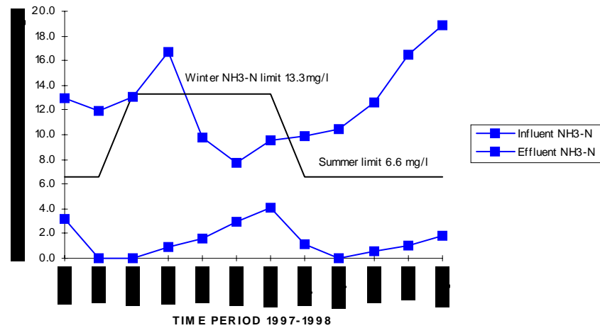
Figure 9D Morganton, NC Monthly Performance Data for Removal of NH 3 -N
