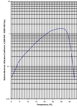
FIGURE 2 Maximum Ammonia Nitrogen Utilization Coefficient, k , as a Function of Temperature for Nitrosomonas
