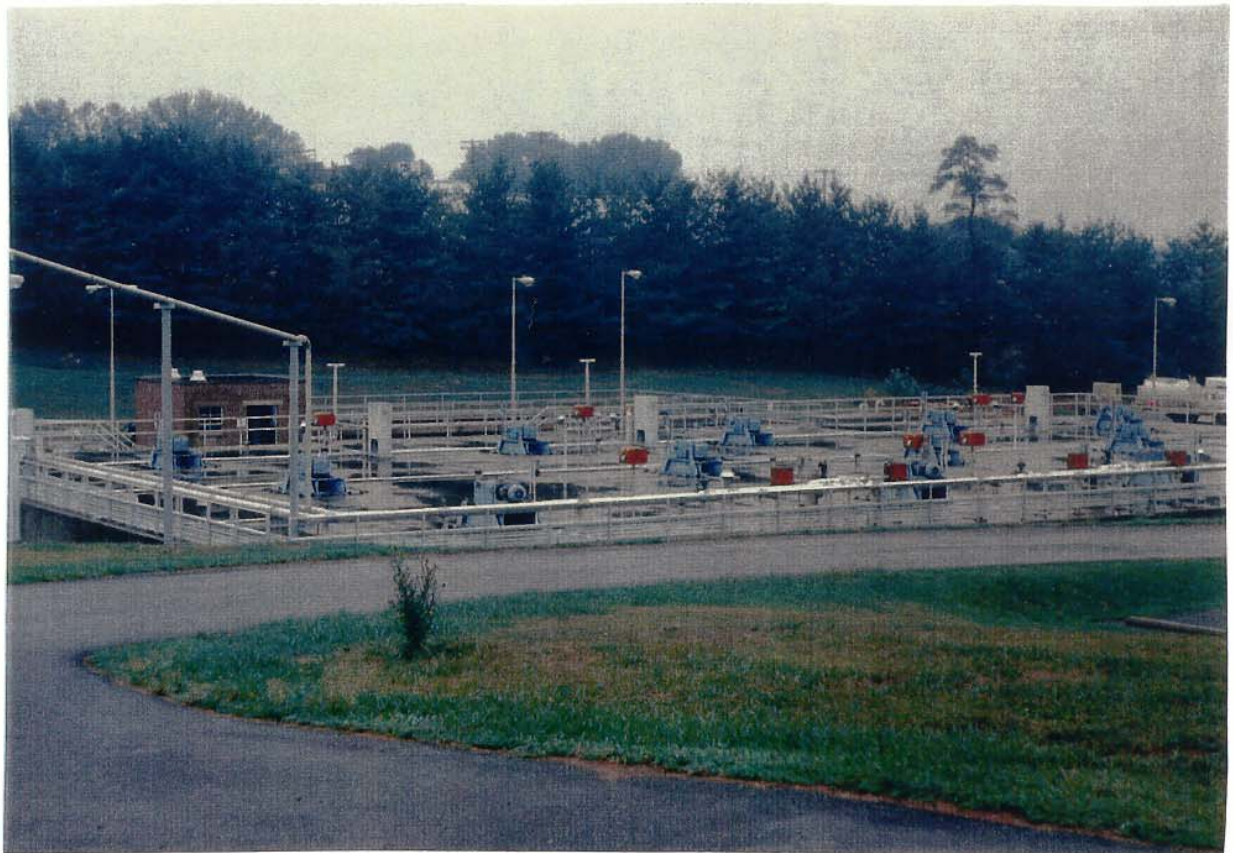
Original UNOX R nitrification reactors
