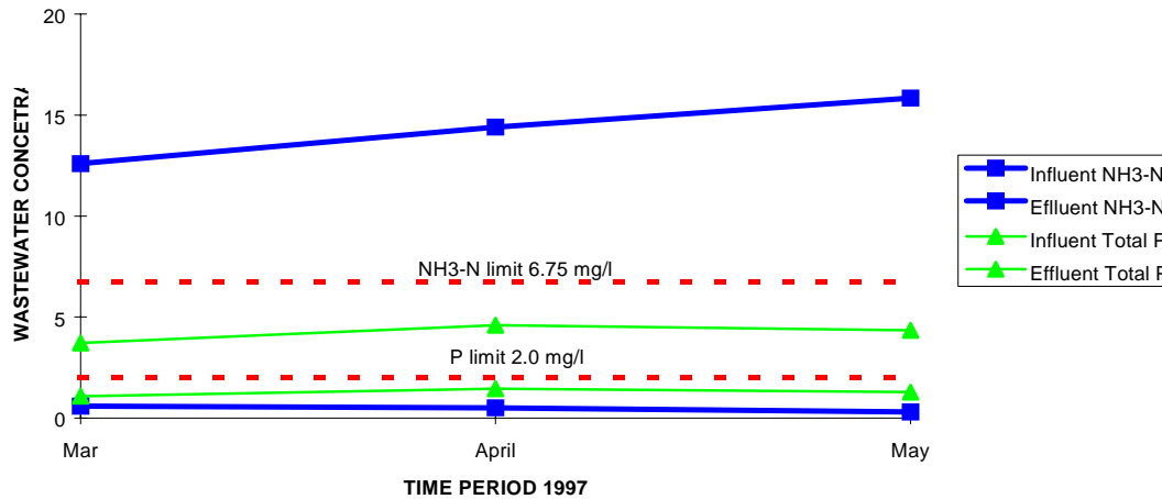
Figure 8 Lancaster, PA Performance Data for Removal of NH 3 -N and Total P
