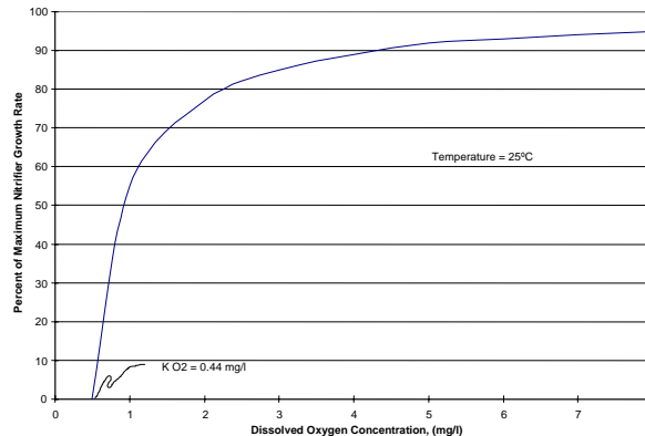
FIGURE 3 Effect of Dissolved Oxygen on the Growth Rate of Nitrifiers
